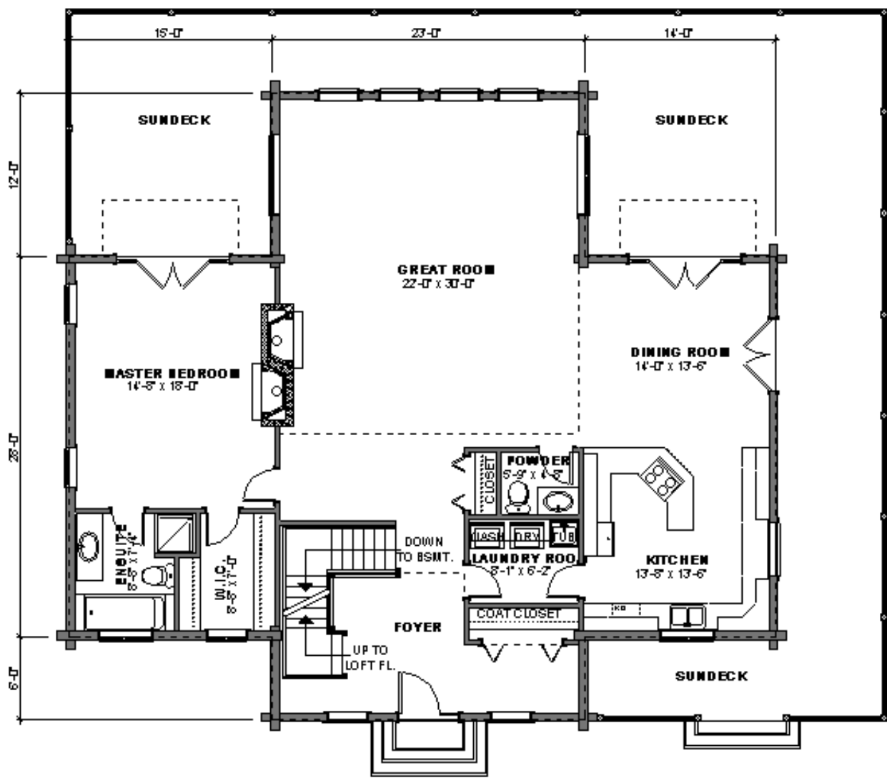
MAIN FLOOR PLAN 1,870 SQ.FT.
