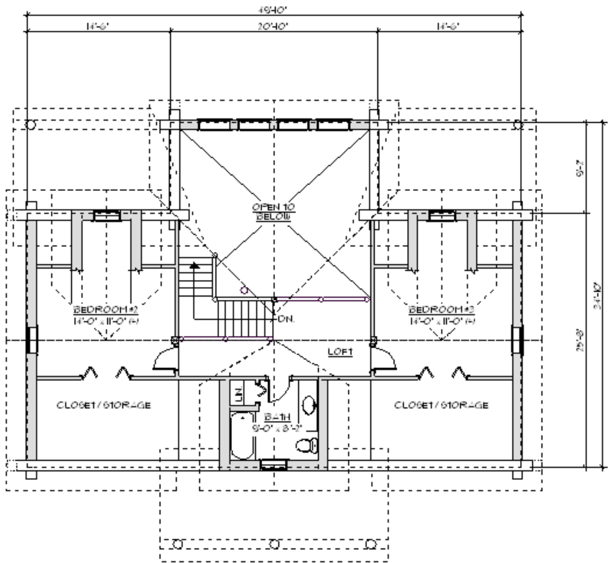
LOFT FLOOR PLAN 103.0 SQ.FT.
