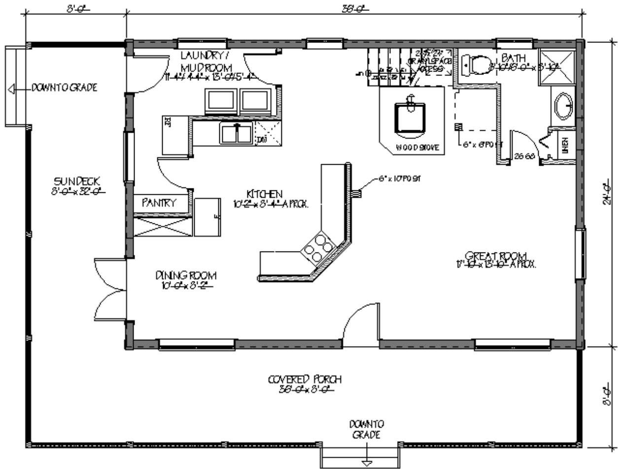
MAIN FLOOR PLAN 864 SQ. FT.
