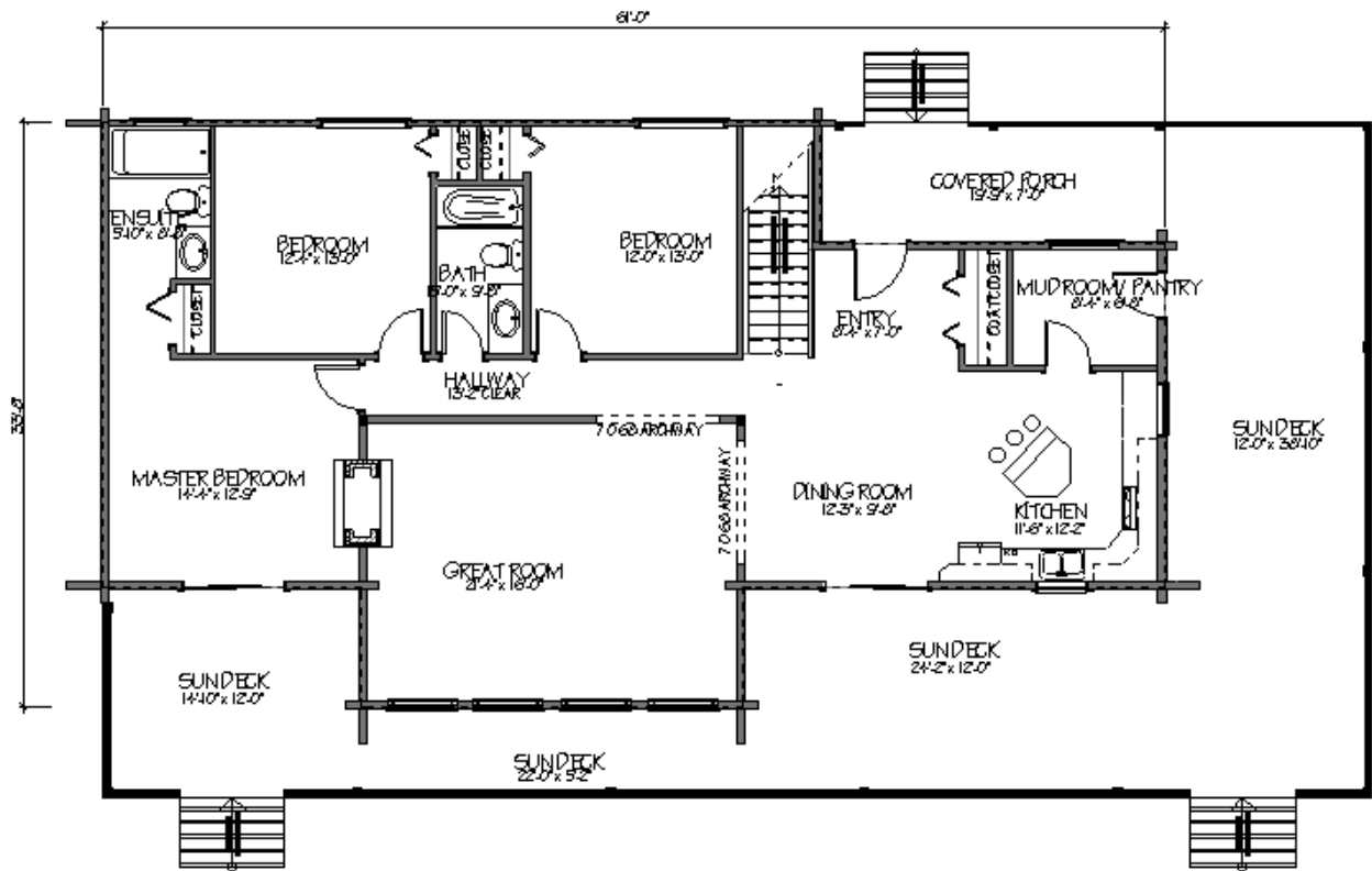
MAIN FLOOR PLAN 1649.3 SQ.FT.
