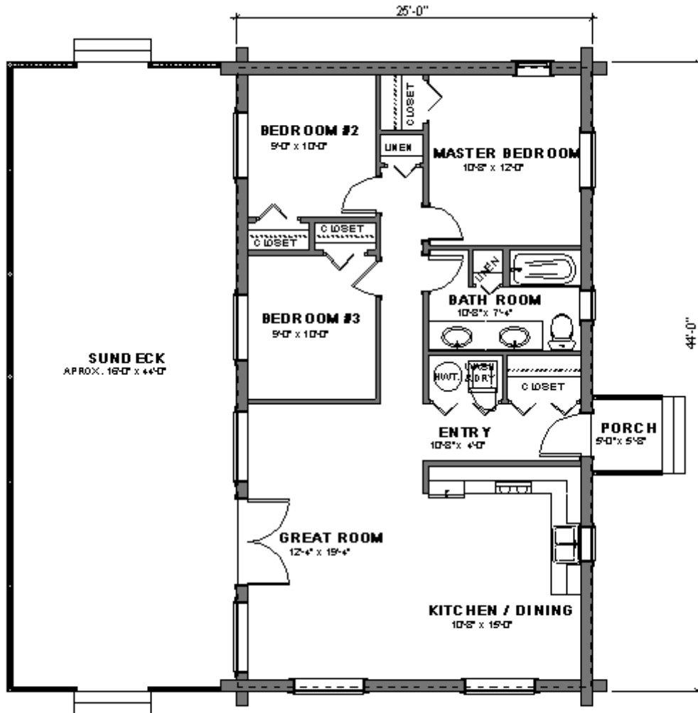
MAIN FLOOR PLAN 1100 SQ.FT.
