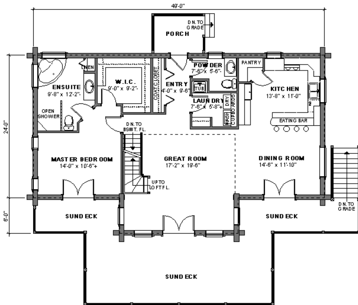
MAIN FLOOR PLAN 1296 SQ.FT.
