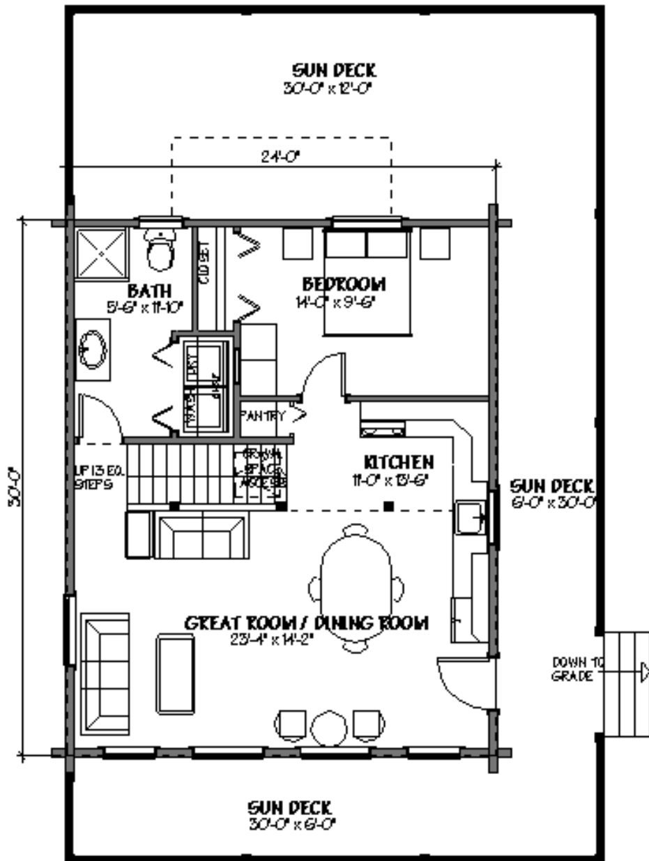
MAIN FLOOR PLAN 720 SQ. FT.
