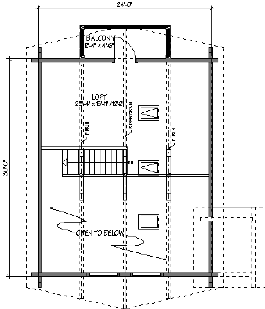
LOFT FLOOR PLAN 345 SQ.FT.
