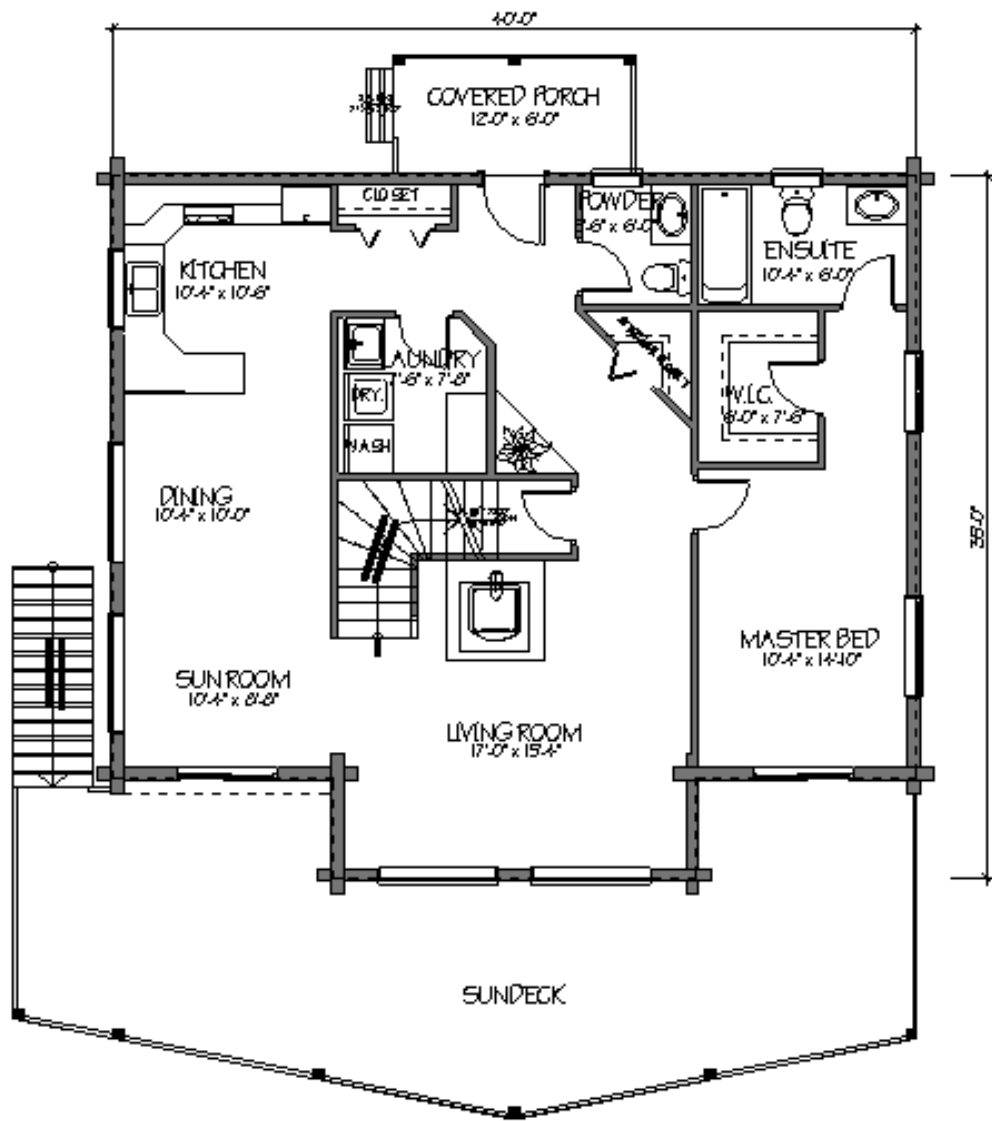
MAIN FLOOR PLAN 1290 SQ.FT
