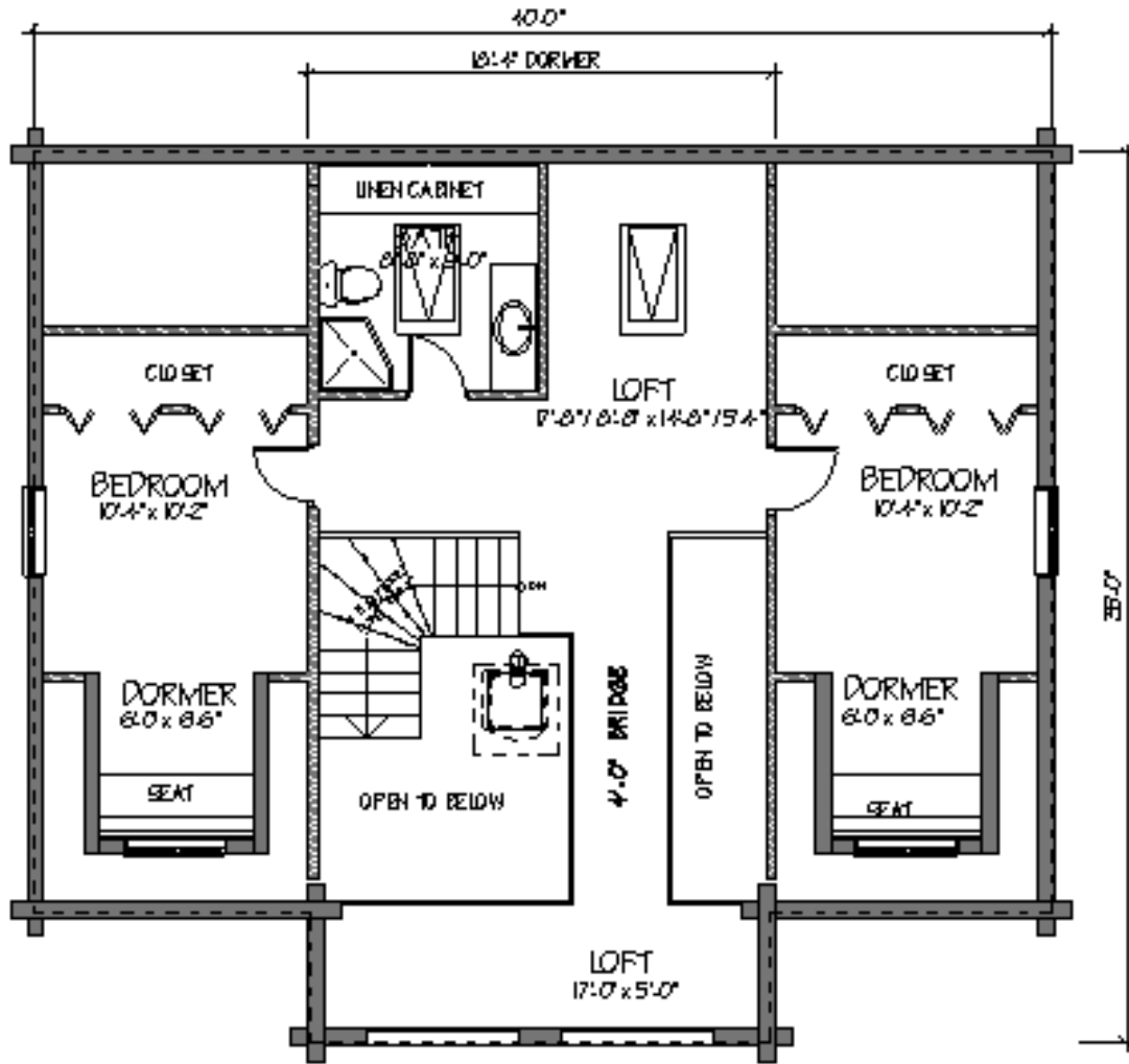
LOFT FLOOR PLAN 801 SQ.FT.
