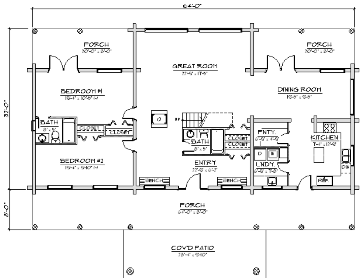
MAIN FLOOR PLAN 1,128.0 SQ. FT.
