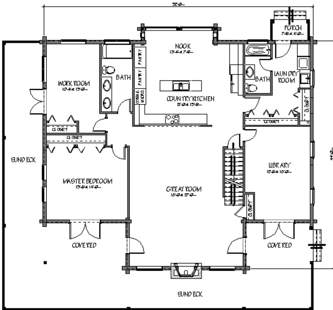
MAIN FLOOR PLAN 2063 SQ. FT. SUNDECK AREA 1083 SQ. FT.
