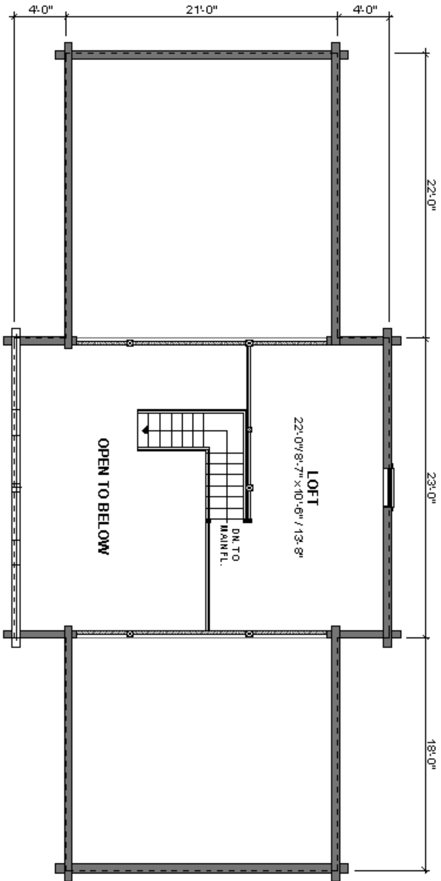
LOFT FLOOR PLAN 280 SQ.FT.
